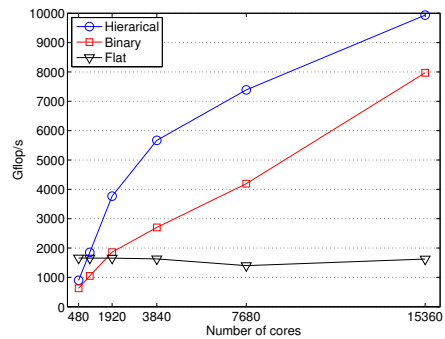
Figure 11. Strong scaling of tree-based QR at (m, n) = (368640, 4608) .
