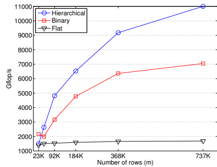
Figure 10. Asymptotic tree-based QR scaling ( n = 4, 608, 9K cores).
